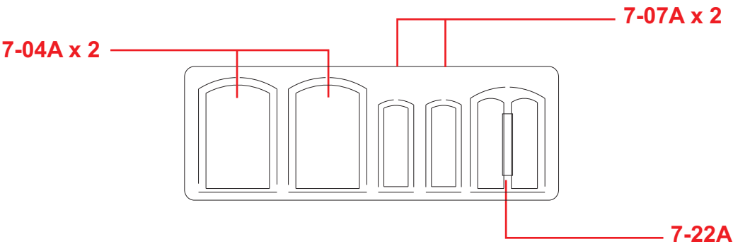
Cartonboard 2mm
